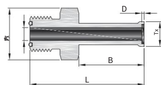
OFS Body to Automatic Tube Weld
