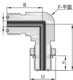
OFS Body to Male SAE/MS Positionable Elbow
