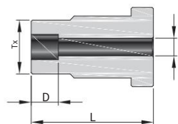
OFS Gland to Tube Socket Weld Reducing
