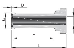
OFS Gland to Automatic Tube Weld
