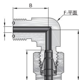
OFS Body to Tube Fitting Elbow
