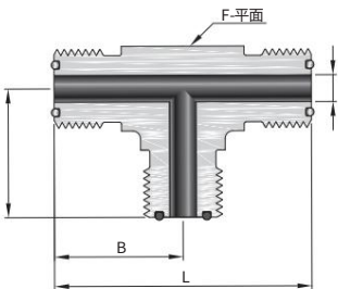
OFS Body Union Tee
