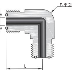
OFS Body Union Elbow
